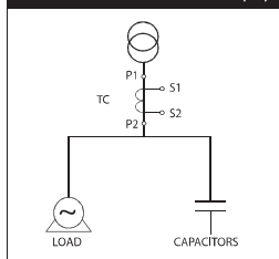
Current Transformer connection (CT)
